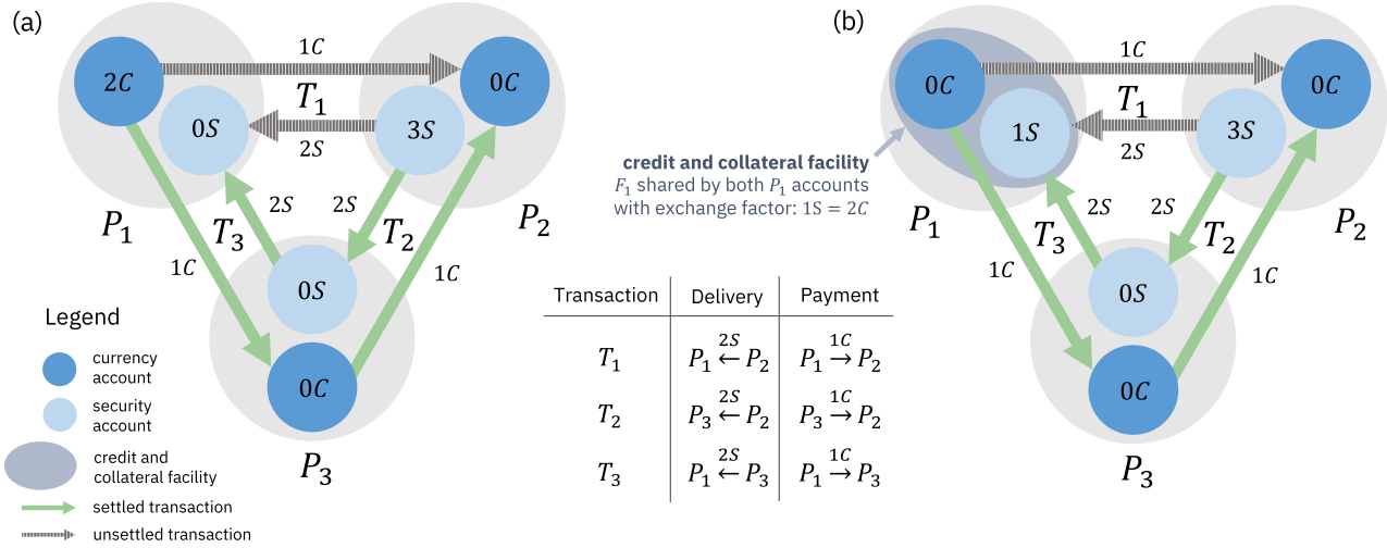
FIGURE 1. Diagrams illustrating a batch of three DvP transactions T_1, T_2, T_3 between three parties P_1, P_2, P_3 . Each party has a currency account C and security account S , with amounts shown in the interior circles. Each transaction is shown with a pair of arrows and the corresponding amount of security and currency involved. In (b), we consider a simplified credit and collateral facility (CCF) (with a net zero amount of credit) shared by both accounts of P_1 , with an exchange factor between currency and security of 1S = 2C . In both (a) and (b), the optimal solution settles transactions T_2 and T_3 , as indicated by the pairs of solid green arrows. With the modification of P_1 's account balances in (b), none of the transactions could settle without the presence of the CCF F_1 , which P_1 can use to convert security into currency to facilitate the transaction with P_3 .
